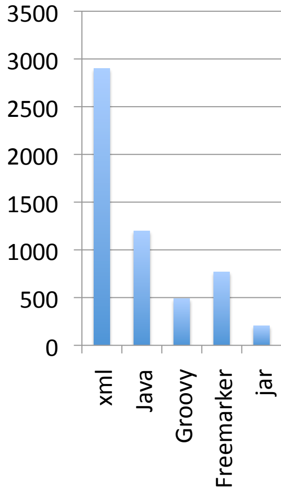
# of files
