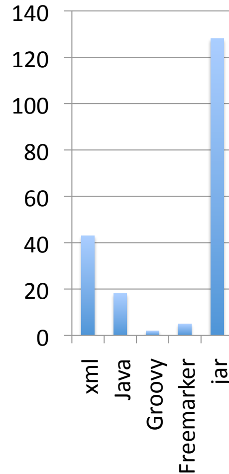
Size (MB)
