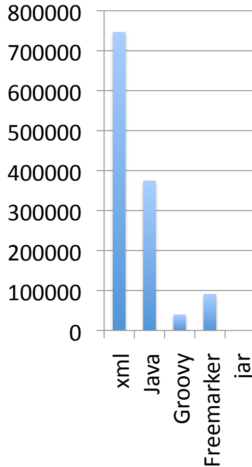
# of Lines
